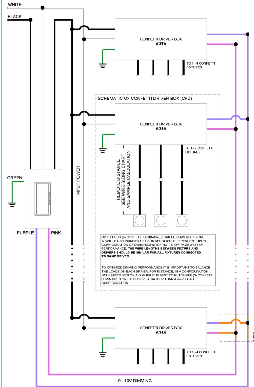
System Wiring Diagram for Confetti Driver Enclosure
